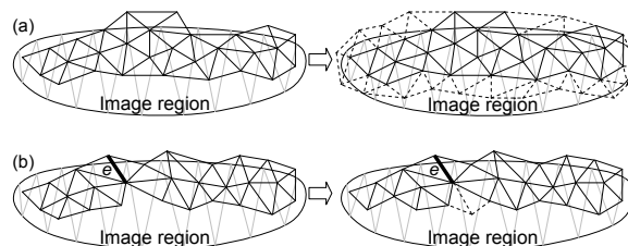
Figure 17. Insertion of triangles.
